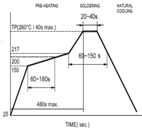
Reflow Soldering
